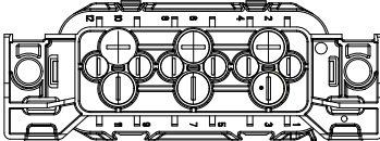
Terminal Numbering (Rear of Unit)
